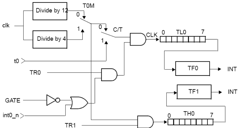
Figure 14 Timer 0 – Mode 3
