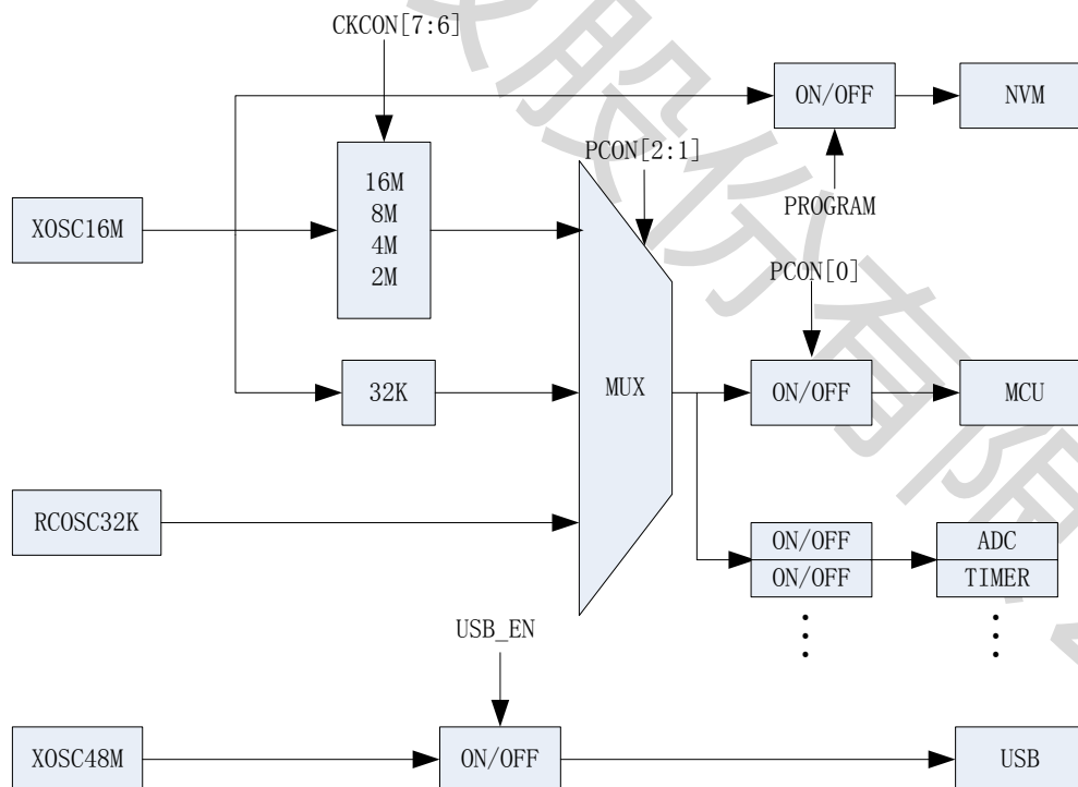
Figure 11 Clock System
