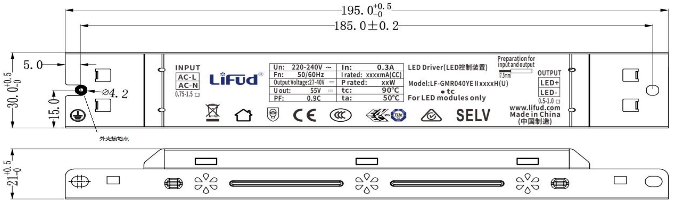
The built-in assembled version
