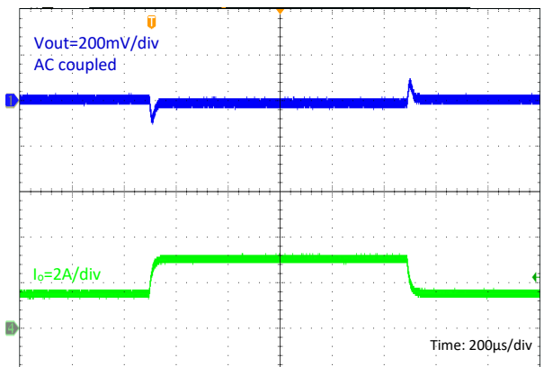
Load Transient
