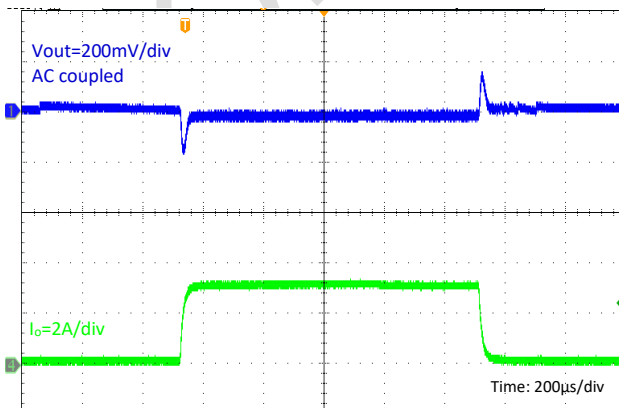
Load Transient
