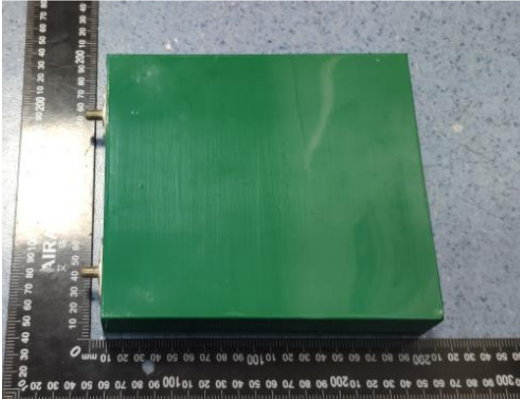
Cells /电芯 (FP45173209A 3.2V 150Ah 480Wh)
