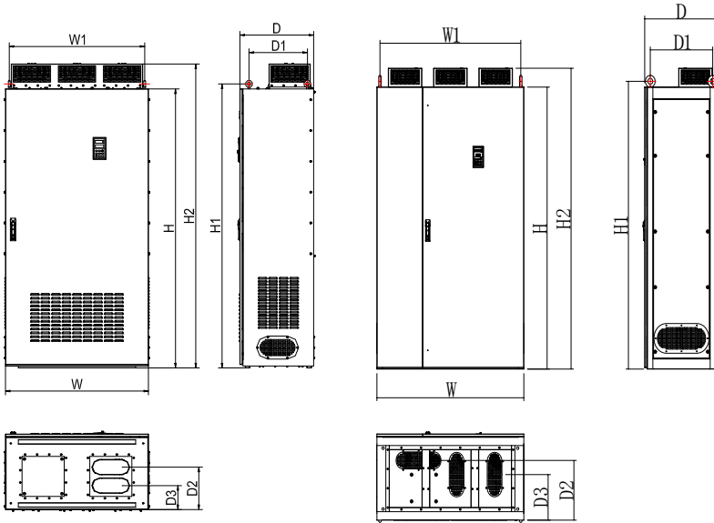
(e) 315KW~630KW 规格尺寸(柜机)
