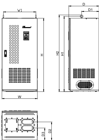
(c) 160KW~200KW 规格尺寸(柜机)
