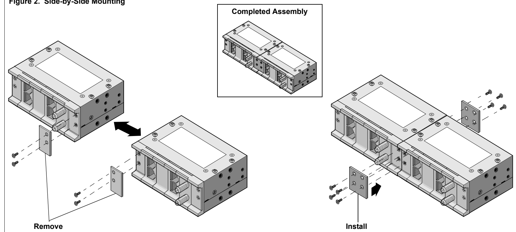
Figure 2. Side-by-Side Mounting
