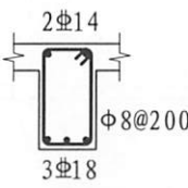
3-3 250 × 450
