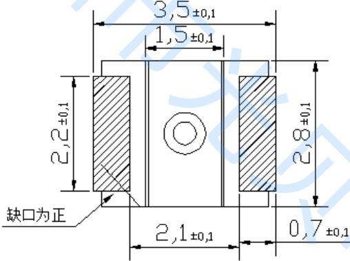
焊盘建议大小 Recommended size of pad
