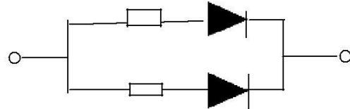
Circuit model B
