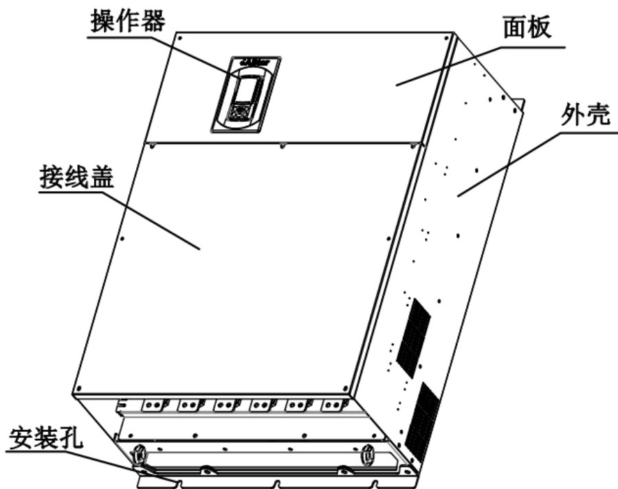
图 2-7 A10~A11
