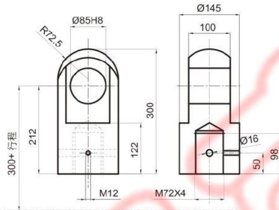
销孔端TF
